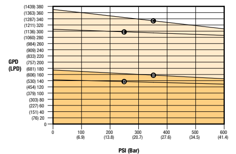
3/4 Inch Plunger
